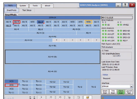
FTB-8115 SmartMode: multichannel signal discovery with real-time alarm scan (shown in the FTB-500 user interface).
