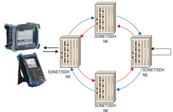
Housed in the FTB-500 or FTB-200 platform, the FTB-8115 module enables field circuit turn-up and troubleshooting.
